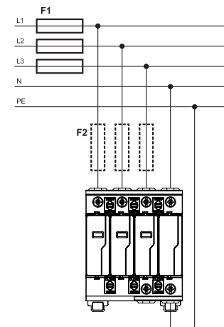
TN-S, TT (3+1)
